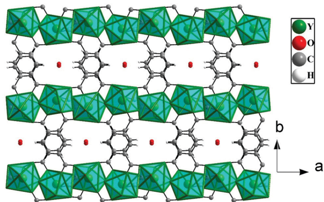
Fig. 2 The connectivity of the 2D structures through terephthalates to form a 3D structure of [\text{Y}(\text{tp})(\text{ox})_{0.5}(\text{H}_2\text{O})_2] \cdot \text{H}_2\text{O} , 1 . Note the presence of 1D water occupying the channels along the c axis. Hydrogen atoms of the water molecules are not shown.
