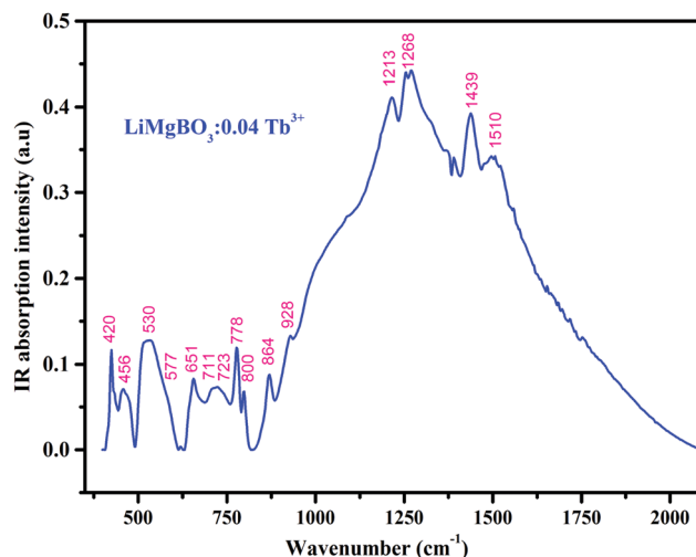
Fig. 4 Infra-red (IR) spectra of \text{LiMgBO}_3:0.04\text{Tb}^{3+}
