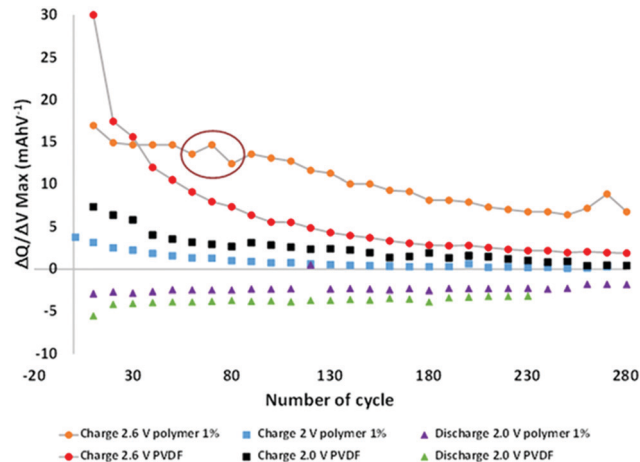
Fig. 3 Maximum derivatives as a function of the number of cycles at different voltages.
