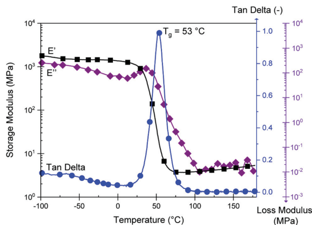
Fig. 5 DMTA data ( -100 \text{ }^\circ\text{C} to 180 \text{ }^\circ\text{C} , 1 \text{ Hz} , 0.1\% strain) of cured CBDA-2 /ELO thermosets using a fixed COOH/oxirane group-ratio of 0.8 (the symbols are intended to help differentiate the curves and do not represent the sole data points).
