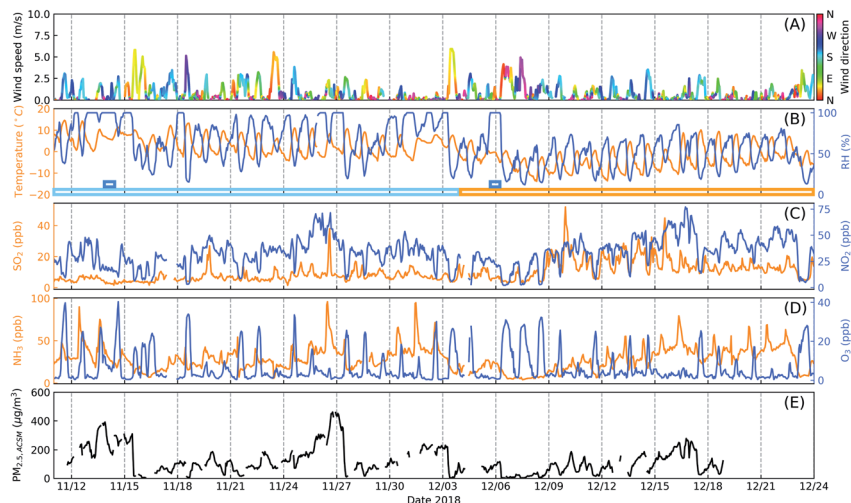
Fig. 1 Time series of meteorological parameters (A and B), inorganic gas pollutants (C and D) and mass concentration of PM_{2.5} (E) during the McFAN campaign. The colored rectangles in panel (B) indicate different characteristic periods: dark blue – fog, light blue – high humidity, orange – low humidity. The mass concentration of PM_{2.5} is obtained by summing up elemental carbon (EC) and other non-refractory aerosol components measured by the OC/EC analyzer and the CV-ToF-ACSM (Table 1), respectively.
