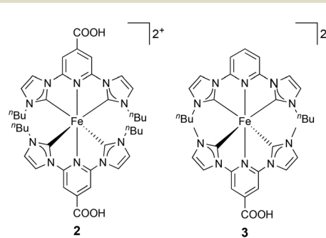
Fig. 2 Structures of the sensitizers 2 and 3 . Both complexes were isolated and used in DSCs as the [PF 6 ] - salts.
