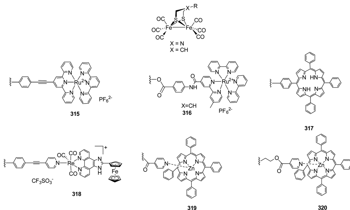
Fig. 109 Models 315 to 320. Examples of \text{Fe}_2(\text{xdt}^{\text{R}})(\text{CO})_6 models modified for photocatalytic purposes.
