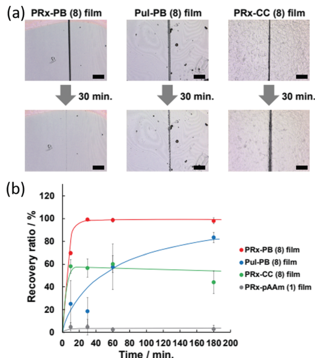
Fig. 31 (a) The self-healing abilities of films containing rotaxanes cross-linked with dynamic boronic acid bonds (PRx-PB), films offering dynamic boronic acid bonds without the additional physical recovery due to rotaxane movement (Pul-PB), and films containing rotaxanes covalently bound to the polyacrylamide backbone (PRx-CC). (b) The recovery ratio versus time of each of the previously described materials, as well as polyrotaxanes with neither dynamic nor covalent crosslinkers (PRx-pAAm). 15 Reproduced from ref. 15 with permission from Cell Press, copyright 2016.
