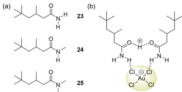
Fig. 21 (a) The structure of ligands 23–25 , reported by Love; (b) extraction of [\text{AuCl}_4]^- is thought to occur via the formation of clusters of one protonated and one neutral ligand.
