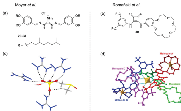
Fig. 23 (a) The structure of receptor 29 , reported by Moyer et al. and (c) X-ray crystal structure of the complex of a simple analogue of DIG with a sulfate anions, showing the dual-coordination by four receptors, one water molecule and one DMSO molecule. Adapted from ref. 17 with permission from The Royal Society of Chemistry; (b) the structure of ion pair receptor 30 , reported by Romański et al. and (d) X-ray crystal structure of the complex of 30 with \text{Na}_2\text{SO}_4 , showing the coordination of the sulfate anion by 4 receptors, forming a charge neutral complex via the inclusion of 2 \times \text{Na}^+ ions in the benzocrown cavities. 17,18 Adapted from ref. 18 with permission from the Royal Society of Chemistry, copyright 2018.
