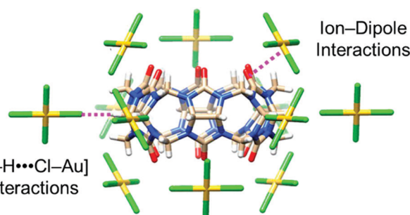
Fig. 20 Stick representation of the X-ray crystal structure of (\text{CB}[6] \cdot [\text{AuCl}_4]^-) , reported by Tao and co-workers. 137 The CB[6] macrocycle is surrounded by 12 [\text{AuCl}_4]^- anions, which form interactions with the outer surface of the macrocycle. Reproduced from ref. 137 with permission from the American Chemical Society, copyright 2020.
