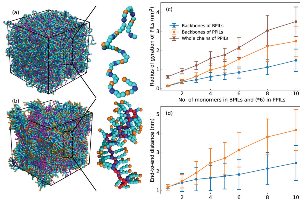
Fig. 16 Representative morphologies and configurations of (a) BPILs and (b) PPILs consisting of 10 and 60 [\text{C}_2\text{C}_8\text{IM}] cation monomers with comparable PIL backbone lengths, and variations of (c) radius of gyration and (d) end-to-end distance of BPILs and PPILs as a function of PIL backbone length. The tail CT beads in cation monomers in BPILs and PPILs, and the head CH beads in PPIL cation monomers are highlighted with orange and red spheres, respectively, to address their spatial distributions in modelling systems.
