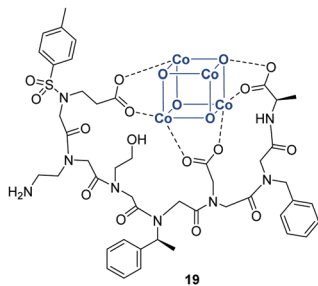
Fig. 6 Hexapeptoid 19 capable to bind the [Co_4O_4] cubane cluster and the pH responsiveness of the respective polymers. The systematic permutation of one building block allowed for investigating a structure-to-function relationship from the peptoid backbone or the respective side-chains. As a result, they found different glass transition and degradation temperatures of polymers in the same mass range (Table 3). 68
