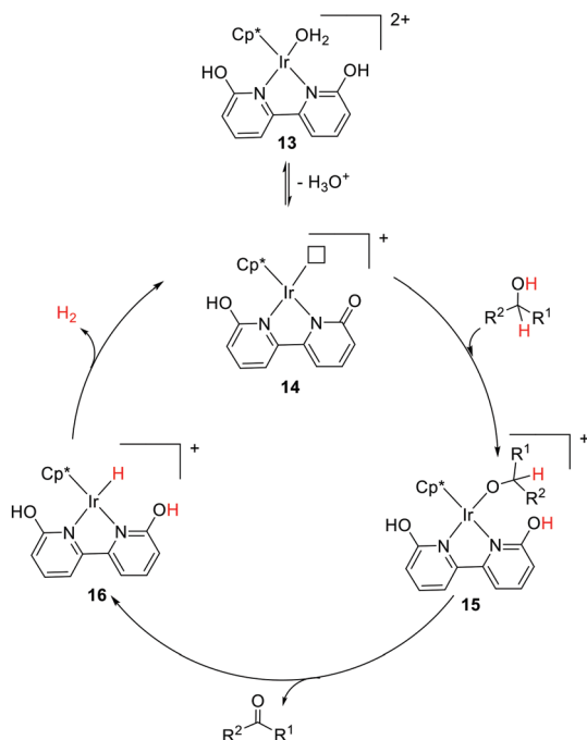
Fig. 9 Proposed mechanistic pathway for alcohol dehydrogenation using the \text{Cp}^*\text{Ir} complex bearing dihydroxy-2,2'-bipyridine.
