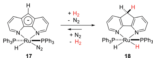
Fig. 10 MLC and \text{H}_2 activation by 4,5-diazafluorenone complex 17 .
