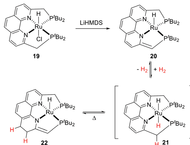
Fig. 11 Reversible \text{H}_2 activation by a Ru phenanthroline-bisphosphine complex (LiHMDS: lithium bis(trimethylsilyl)amide).
