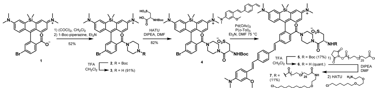
Scheme 2 Synthesis of isoBeRST-pipycys ( 6 ) and isoBeRST-Halo ( 7 ).
