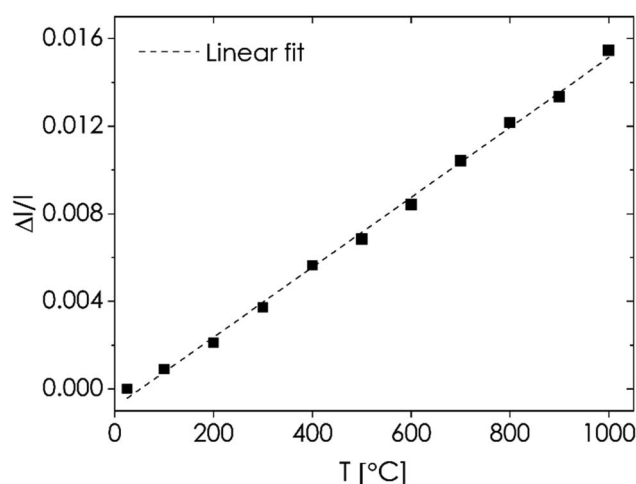
Fig. 6 Relative thermal expansion for \text{La}_{0.7}\text{Sr}_{0.3}(\text{Co},\text{Cr},\text{Fe},\text{Mn},\text{Ni})\text{O}_{3-\delta} obtained from structural data.
