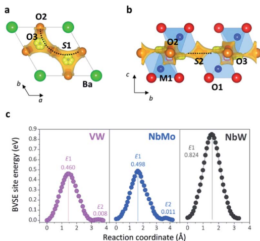
Fig. 7 BVSE map of Ba 3 VWO 8.5 showing the 2-dimensional ionic conduction pathway along the palmierite-like layer as seen down the c -axis (a) and a -axis (b). Isosurface levels are drawn at < 0.5 eV (over the global minimum). The dotted lines represent the saddle points as identified by the softBV software. (c) BVSE models of migration barriers along the palmierite-like layers for Ba 3 VWO 8.5 (VW), Ba 3 NbMoO 8.5 (NbMo), and Ba 3 NbWO 8.5 (NbW). Relative bond-valence energy barriers are reported in eV. Note that the minimum site energies have relative values.
