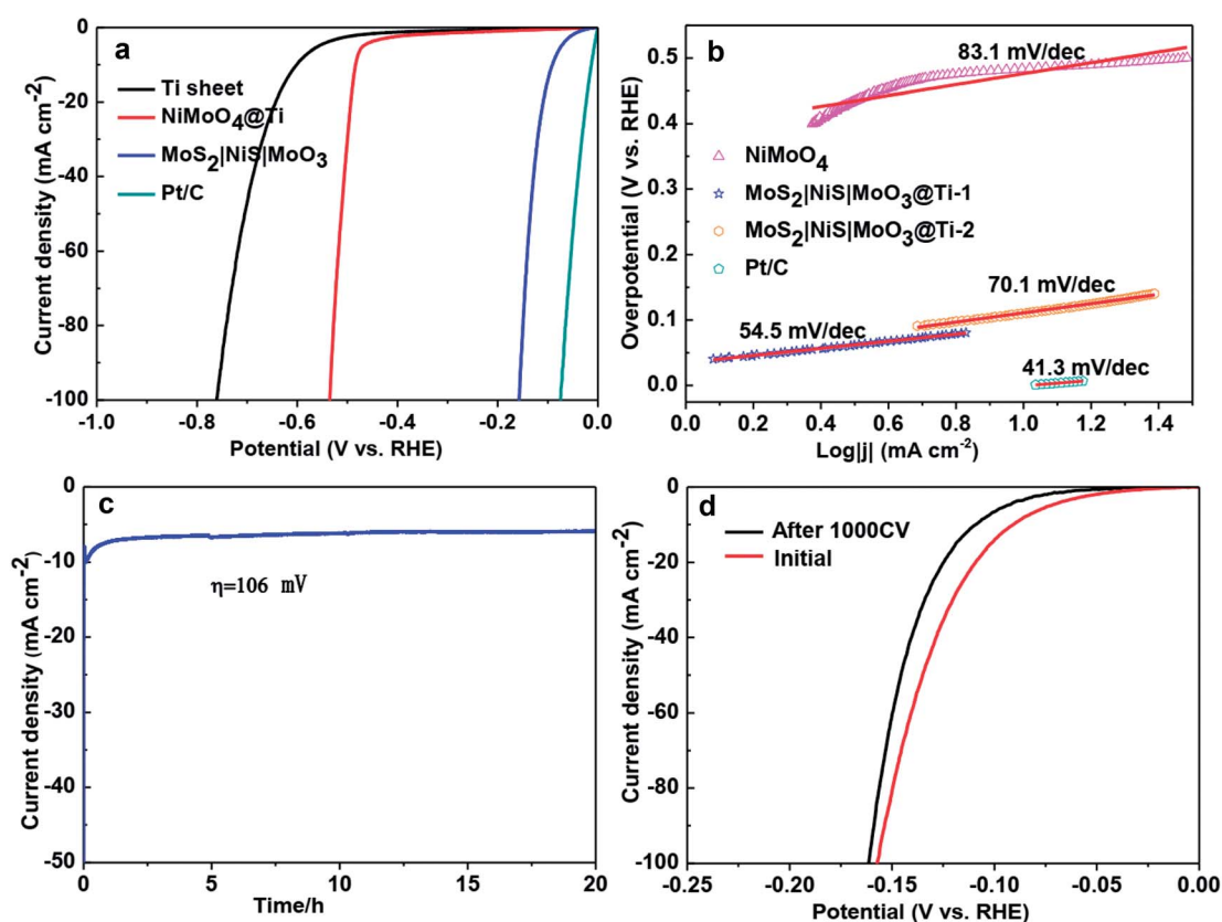
Fig. 4 (a) HER LSVs of \text{MoS}_2\text{[NiS]/MoO}_3\text{/Ti} foil in comparison with other studied electrodes in 1 M KOH. (b) Corresponding Tafel plots. (c) CA response of \text{MoS}_2\text{[NiS]/MoO}_3\text{/Ti} foil for more than 20 h. (d) HER LSVs of \text{MoS}_2\text{[NiS]/MoO}_3\text{/Ti} foil before and after 1000 CV cycles. Reproduced with permission from ref. 60 (Copyright 2017 American Chemical Society).
