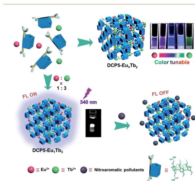
Fig. 1 Schematic illustration of the construction of the color-tunable pillarene coordination polymer (PCP), i.e., DCP5- \text{Eu}_x\text{Tb}_y , simply by tuning the molar ratio of \text{Eu}^{3+} and \text{Tb}^{3+} in the system and the fluorescence ON/OFF sensing of nitroaromatic pollutants by a typical PCP, i.e., DCP5- \text{Eu}_1\text{Tb}_3 .
