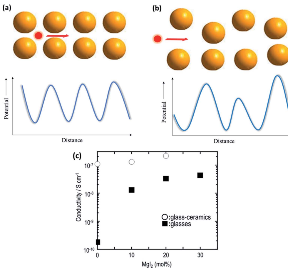
Fig. 8 Potential energy landscape for (a) crystalline and (b) amorphous materials for the transport of ions; (c) plot of ionic conductivity as a function of \text{MgI}_2 concentration in 60\text{MgS}-40\text{P}_2\text{S}_5 parent glass. Reproduced from ref. 123 with permission, copyright 2014, Elsevier.
