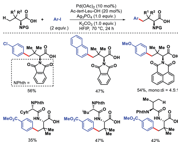
Scheme 54 Pd catalyzed \gamma\text{-C}(\text{sp}^3)\text{-H} arylation of tert -leucine and its derived peptides.
