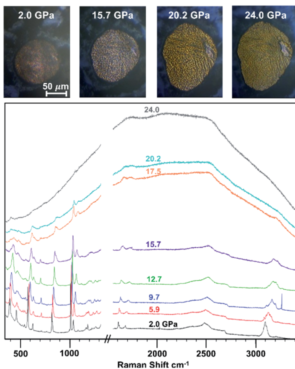
Fig. 2 In situ Raman spectral overlay depicting 1:1 phenol : pentafluorophenol co-crystal throughout compression. The top images are taken with the Raman microscope during compression.
