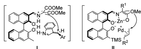
Scheme 30 Asymmetric nucleophilic substitution catalyzed by binaphthyl derived catalyst.
