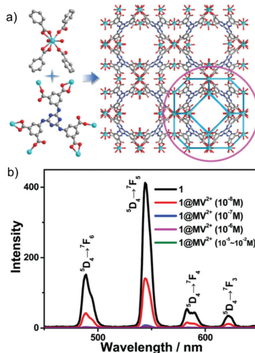
Fig. 15 (a) Coordination environment of the \text{Tb}^{3+} ions and the coordination model of the TATAT 6- ligands in the three-dimensional structure of the MOF. (b) Solid-state emission spectra of the MOF and soaked samples of the MOF in \text{MV}^{2+} aqueous solutions with different concentrations. Reproduced with permission from ref. 131. Copyright 2018 Royal Society of Chemistry.
