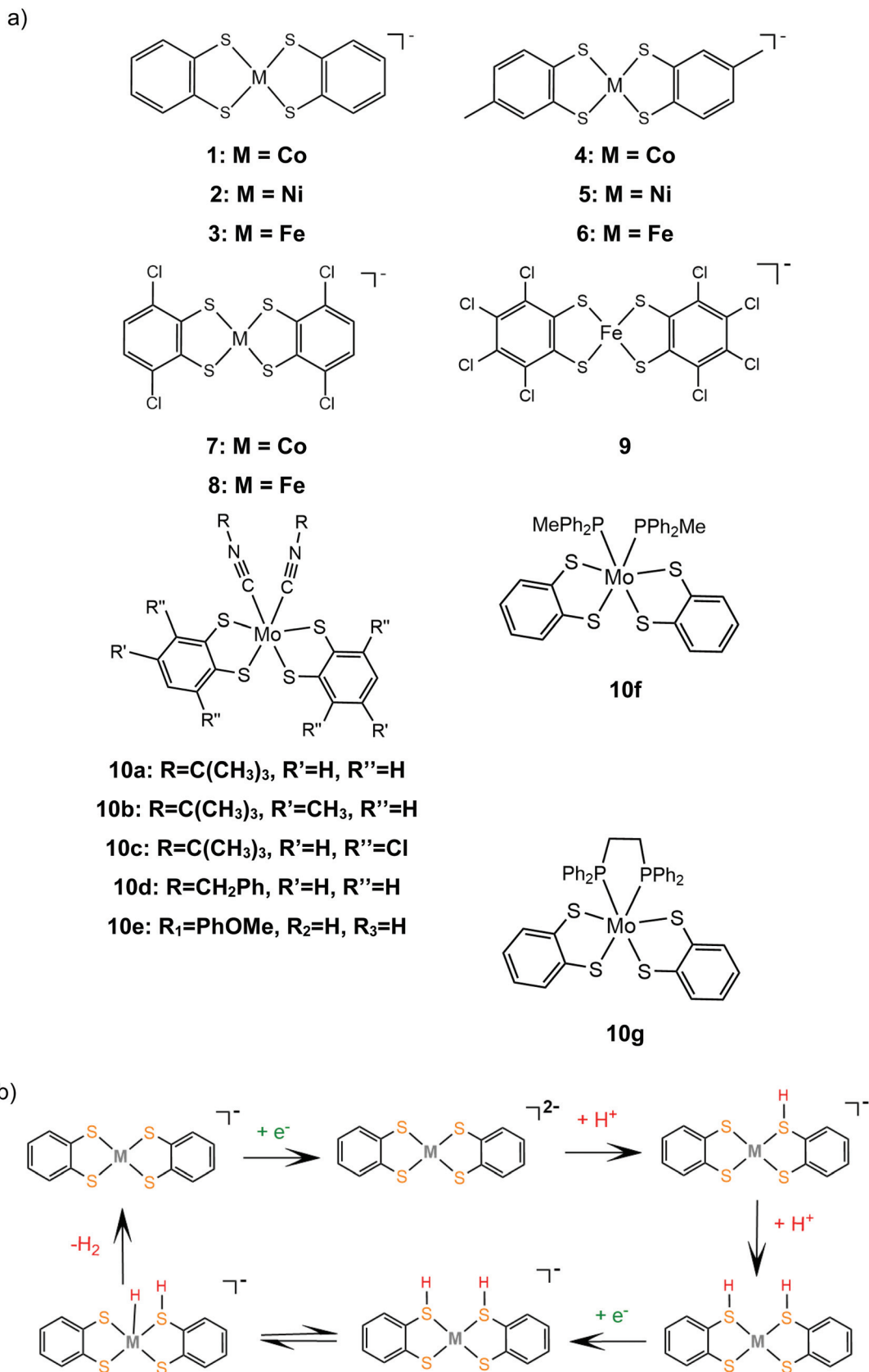
Scheme 7 (a) Metal complexes [M(bdt) 2 ] acting as HER catalysts. (b) Proposed ECCE mechanism catalysed by complexes 1 , 2 and 3 .
