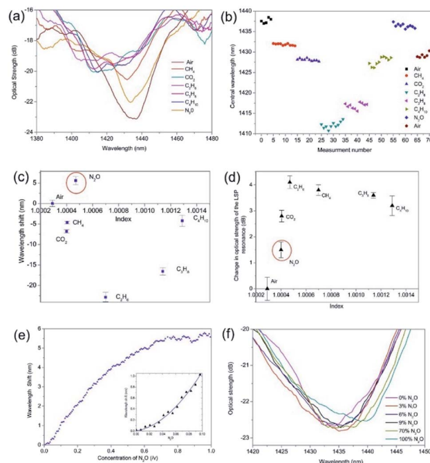
Fig. 7 The typical experimental results of a UV processed \text{Ge}/\text{SiO}_2/\text{Pt} LSP fibre device coated with SWNTs and PEI as a function of surrounding refractive index and the detection of nitrous oxide (a) the transmission spectra as function of changing surrounding index and the nitrous oxide. (b) The individual measurements of the central wavelength of the LSP resonance for each alkane gas and nitrous oxide (c) and (d) the wavelength and optical strength sensitivity as a function of the different gases and their refractive index respectively. (e) The wavelength response to increasing \text{N}_2\text{O} concentration, the insert showing the wavelength shift with low concentrations of \text{N}_2\text{O} . (f) Examples of the changes in transmission spectra of LSP resonance to various concentrations of \text{N}_2\text{O} as a percentage of total volume.
