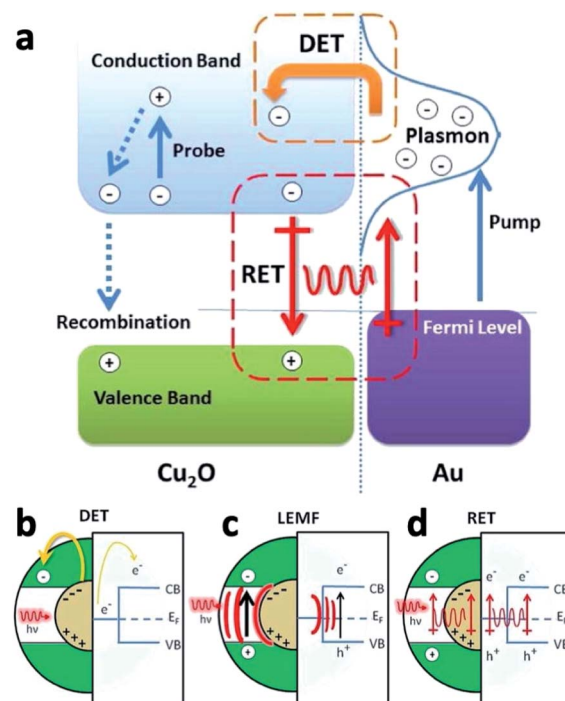
Fig. 14 Various possible energy-transfer and separation processes responsible for plasmon-enhanced photocatalytic activity of \text{Cu}_2\text{O}/\text{Au} -based HNS. 125 (a) Scheme of energy absorption at the metal (pump) and the subsequent energy-transfer processes: (b–d) illustration of the metal core (Au) and the SC shell ( \text{Cu}_2\text{O} ) energy positions (right) and processes (left): (b) direct energy transfer (DET), where LSPR 'hot' electrons are transferred to the SC's CB; (c) local electromagnetic field enhancement (LEMF), where the e^- – h^+ charge-separation in the SC is radiatively aided by the metal excitation; (d) resonant energy transfer (RET), where the LSPR dipole induces e^- – h^+ pair separation in the SC via a non-radiative mechanism that relaxes the localized surface plasmon dipole. Adapted with permission from the American Chemical Society, copyright 2012.
