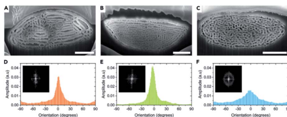
Fig. 4 The Sulawesiella rafaélæ longhorn beetle displays orange (A and D), green (B and E) and turquoise (C and F) coloured areas due to perforated multilayer structures embedded in the scales covering the beetle elytra. Based on SEM images of the scale cross-sections (A–C), variable distributions in the layer orientations (D–F) were measured and 2D-FFT analyses were performed (insets in D–F). The different extents of disorder in these scales give rise to various iridescence and scattering properties. Scale bars: 2 \mu\text{m} (A–C). Reproduced from ref. 52, License CC-BY-NC-ND.
