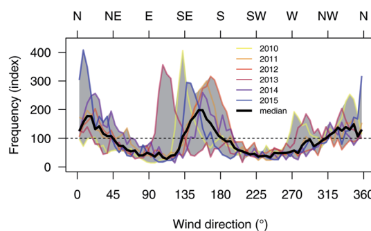
Fig. 1 Wind direction frequencies during ice-off periods 2010–2015 at Toolik Lake. The frequency index 100 indicates the expectation value of a uniform distribution of wind directions. The gray band shows the range of all six years, the bold line is the median from all years. Note that the measurement platform mooring was not rigid, and thus the shift in peak wind directions in the E–S sector rather reflects the differences in configuration of the platform mooring during individual summers, and most likely is not indicating a real difference in wind directions.
