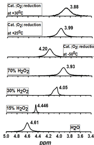
Fig. 5 ^1\text{H} -NMR spectra of the products formed during the complex \text{Co}_4\text{L1} catalyzed dioxygen reduction reactions at 25 °C, 30 °C and -50 °C [ \text{Co}_4\text{L1} (0.01 mM), \text{Fc}^* (3 mM), TFA (10 mM) and \text{O}_2 (0.18 mM)] in acetone- d_6 and comparison with authentic samples containing 70%, 30%, 15% and 0% (weight percent \text{H}_2\text{O}_2 basis) \text{H}_2\text{O}_2/\text{H}_2\text{O} mixtures. All the ^1\text{H} -measurements were performed at 25 °C. The results obtained for \text{Co}_4\text{L1} are then compared with that for \text{Co}_6\text{L2} in Table 2.
