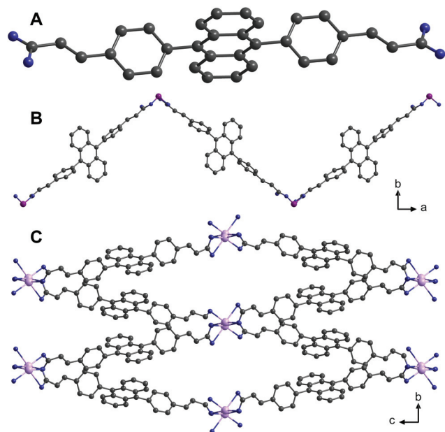
Fig. 1 Solid-state structures of (A) H 2 L, (B) one-dimensional coordination polymer [Zn(L)(DMF) 2 ] n (1) and (C) a three-dimensional metal-organic framework [Cd(L)(DMF)]·DMF n (2) based on 4,4'-(9,10-anthracenediyl)dicinnamic acid (H 2 L). Solvent molecules and hydrogen atoms were omitted for clarity. Colour code: C, black; O, blue; Zn, purple; Cd, pink.
