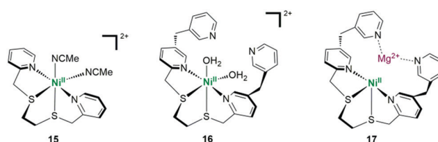
Fig. 14 Ni complexes for \text{CO}_2 photoreduction bearing an \text{S}_2\text{N}_2 -type tetradentate ligand as the photocatalyst and a Ni(II) complex bearing an \text{S}_2\text{N}_2 -tetradentate ligand with two noncoordinating pyridine pendants as the photocatalyst.
