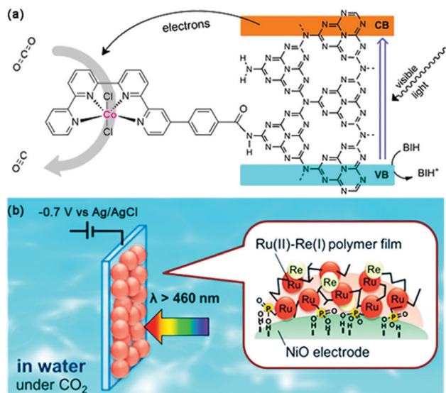
Fig. 16 (a) Visible-light-driven CO 2 reduction by a cobalt complex covalently linked to mesoporous carbon nitride. Reprinted with permission from ref. 121. Copyright 2020 American Chemical Society. (b) PolyRuRe/NiO photocathode for CO 2 photoreduction. Reprinted with permission from ref. 124. Copyright 2019 American Chemical Society.
