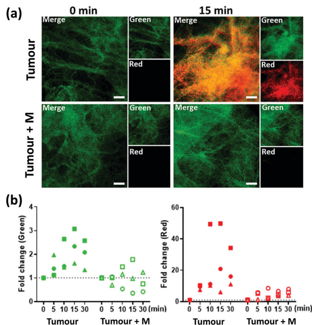
Fig. 2 Specific activation of 3 by cancerous human lung tumour tissue. Compound 3 ( 5\text{ }\mu\text{M} ) was added to ex vivo human lung cancer tissue ( \pm marimastat, M). The tissue was interrogated using an optical fibre-based imaging device with 300 frames collected per time-point (0–30 min) post addition of 3 . (a) Individual frame from the 10 s video (per time-point/condition) is shown. Merge is an overlay of the two fluorescent channels, which are shown individually within the inserts. (b) Fold-change in average fluorescence (FAM: green and Cy5.5: red) after incubation with the compound was compared to base-line fluorescence from the two channels. At each time point, the mean intensity of the 300 video frames is shown. Data is from three independent patient tumour samples with each symbol representing an individual patient ( \pm marimastat, M). Scale bar is 50\text{ }\mu\text{m} .
