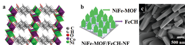
Fig. 4 (a) The overall crystal structure of ultrathin MOF nanosheets of \text{NiCo-MOF} ( \text{NiCo-UMOFNs} ), with three coordination structural layers. Reprinted with permission from (ref. 34). Copyright (2016) Springer Nature. (b) A representative diagram of the fabrication of \text{NiFe-MOF/FeCH-NF} . (c) SEM image of \text{NiFe-MOF/FeCH-NF} . Adapted with permission from ref. 133 with the permission of The Royal Society of Chemistry.
