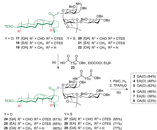
Scheme 2 Reagent and conditions: (a) EtOCOCI, \text{Et}_3\text{N} , THF, 0 °C to r.t., 4 h, 61% (for 24 ), 65% (for 25 ), 90% (for 26 ); 65% (for 27 ), 71% (for 28 ), and 77% (for 29 ); (b) 1: Pd/C, \text{H}_2 (1 atm), EtOH/THF 1 : 1, r.t., 16 h (for 24-26 ); 20 min (for 27-29 ); 2: TFA/ \text{H}_2\text{O} 3 : 1, 0 °C, 1 h, 84% (for 3 ), 49% (for 4 ), 63% (for 5 ); 46% (for 6 ), 36% (for 7 ), and 23% (for 8 ).
