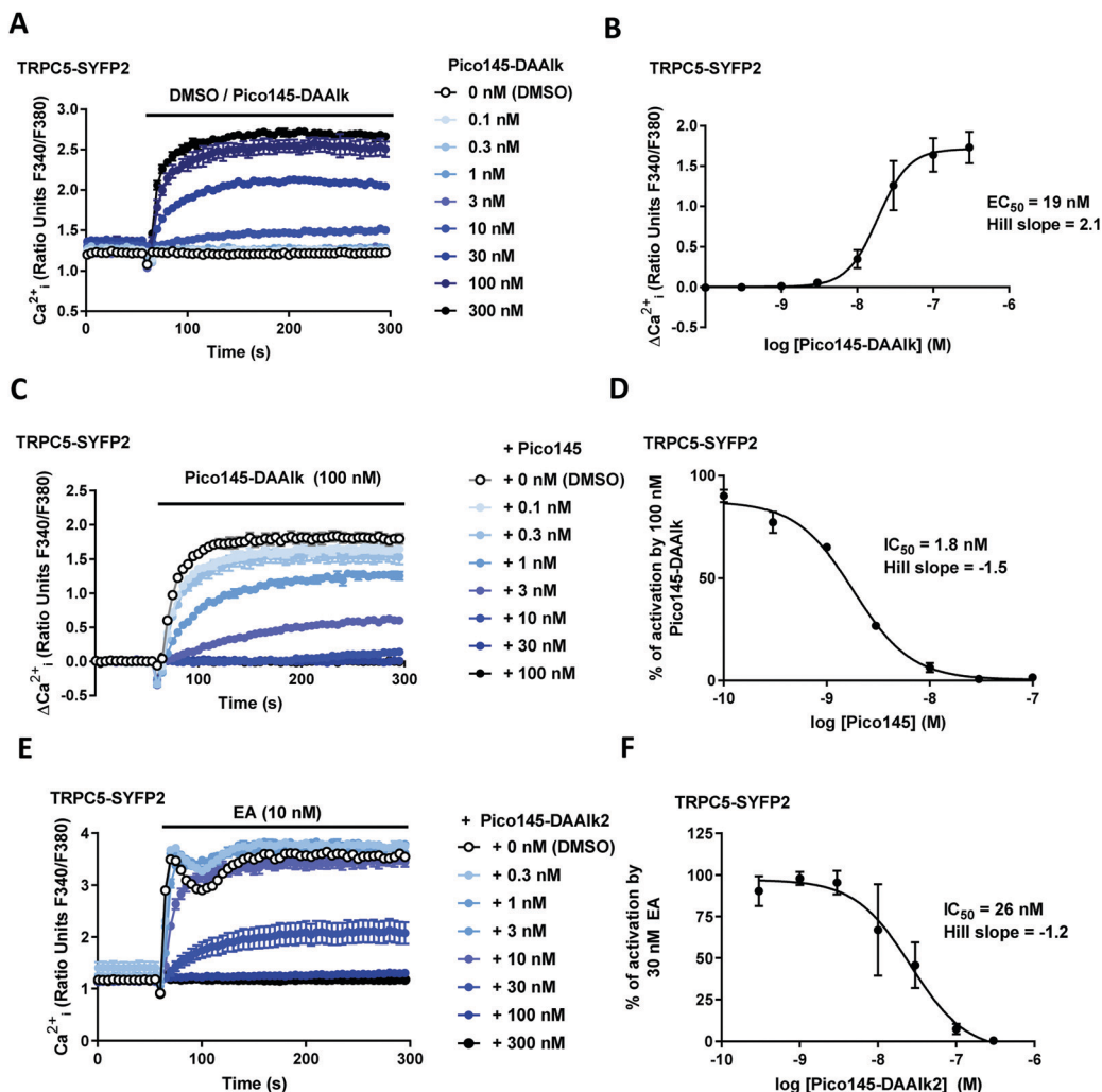
Fig. 2 Pico145-DAAlk 5 and Pico145-DAAlk 2 are potent TRPC5:C5 channel modulators. (A) Representative traces from a single 96-well plate ( N = 6 ) showing an increase in [\text{Ca}^{2+}]_i in response to 0.1–300 nM Pico145-DAAlk 5 in (Tet+) HEK T-REx cells overexpressing hTRPC5-SYFP2. (B) Concentration–response data for experiments in (A), showing mean responses \pm SEM ( n/N = 3/18 ). Responses were calculated at 150–200 s, compared to baseline at 0–55 s. (C) Representative traces from a single 96-well plate ( N = 6 ) showing an inhibition by 0.1–100 nM Pico145 1 of the increase in [\text{Ca}^{2+}]_i in response to 100 nM Pico145-DAAlk 5 in (Tet+) HEK T-REx cells overexpressing hTRPC5-SYFP2. (D) Concentration–response data for experiments in (C) showing mean responses \pm SEM ( n/N = 3/18 ). Responses were calculated at 150–200 s, compared to baseline at 0–55 s. (E) Representative traces from a single 96-well plate ( N = 6 ) showing an inhibition by 0.3–300 nM Pico145-DAAlk 7 of the increase in [\text{Ca}^{2+}]_i in response to 10 nM EA in (Tet+) HEK T-REx cells overexpressing hTRPC5-SYFP2. (F) Concentration–response data for experiments in (E), showing mean responses \pm SEM ( n/N = 3/18 ). Responses were calculated at 250–295 s, compared to baseline at 0–55 s.
