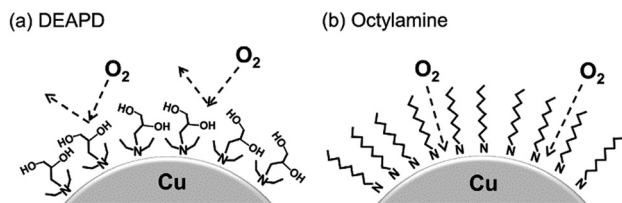
Fig. 2 Adsorption model of (a) 3-diethylamino-1,2-propanediol (DEAPD) and (b) octylamine on a copper particle. Reproduced with permission from ref. 92. Copyright 2014, Elsevier.
