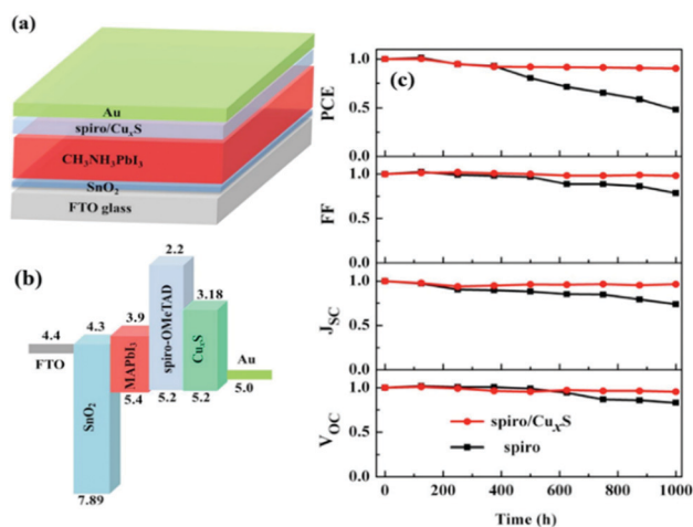
Fig. 14 (a) Schematic illustration of the device structure of a planar n-i-p MAPbI 3 solar cell, with the spiro-OMeTAD/ \text{Cu}_x\text{S} bilayer; (b) energy band diagram of the PSC; (c) PCE, FF, J_{SC} , and V_{OC} as a function of ambient storage time of devices with different HTLs. 114
