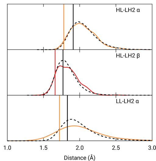
Fig. 5 Hydrogen bond length distributions for \alpha Bchl-Trp45 and \beta Bchl-Tyr44 of HL-LH2 and for \alpha Bchl-Tyr41 of LL-LH2 along the MD compared with the results from the full optimization from previous work (black sticks) 25 and from the present constrained optimization (colored sticks) of the BChls. We reported the distribution from the whole MD (18 000 frames) as a black dashed line and from the 50 frames selected for excitonic calculations as a colored line.
