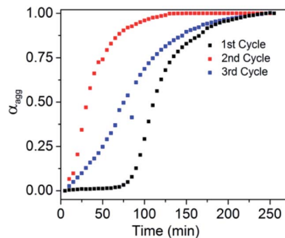
Fig. 6 Variation of \alpha_{agg} vs. time for living SROP; 2.5% DMAP was used in the first cycle while NDI-1 sp (NDI-1 mono /NDI-1 sp = 34) was used in the 2 nd and 3 rd cycles.
