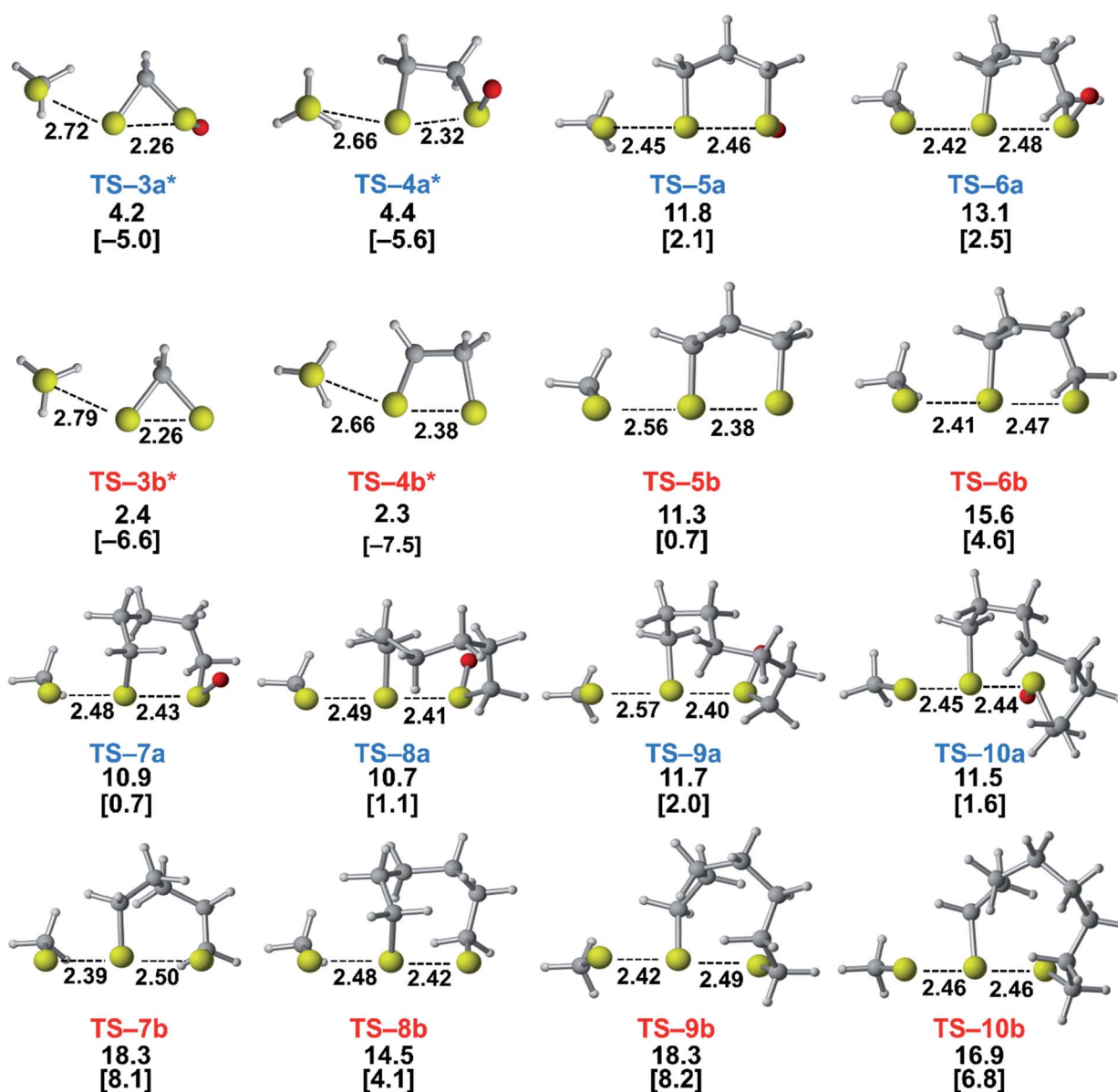
Fig. 1 Transition structures for the reaction of \text{MeS}^- with cyclic thiosulfonates (3–10)a and cyclic disulfides (3–10)b. The \Delta G^\ddagger and \Delta H^\ddagger (in brackets) were computed with M06-2X/6-311++G(d,p) IEF-PCM ^{\text{H}_2\text{O}} and provided for each transition structure. The bond lengths and energies are reported in Å and kcal mol ^{-1} , respectively. *We were unable to locate transition states for (3–4)a and (3–4)b using B3LYP-D3BJ, M06-2X, or MP2 methods. Reported structures are energies for a constrained transition structure featuring one negative frequency corresponding to the substitution reaction using M06-2X/6-311++G(d,p).
