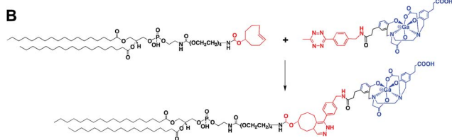
Fig. 4 (A) Radio-HPLC chromatograms of (top) [^{68}\text{Ga}]\text{Ga-HBED-CC-tetrazine} precursor and (bottom) reaction between 4 and 5, after 15 min at 60 ^{\circ}\text{C} . (B) Scheme of the reaction between TCO-modified PE (4) and [^{68}\text{Ga}]\text{Ga-HBED-CC-tetrazine} (5).
