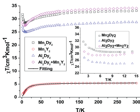
Fig. 3 Temperature dependence of the \chi T product at 300 Oe for 3 \{\text{Mn}_2\text{Dy}_2\} , 4 \{\text{Mn}_2\text{Y}_2\} (the solid line is the best fit to the experimental data for 4). The comparison curves (inset) of \{\text{Mn}_2\text{Dy}_2\} and \{\text{Al}_2\text{Dy}_2\} + \{\text{Mn}_2\text{Y}_2\} along with the curves of 4 \{\text{Mn}_2\text{Y}_2\} and 7 \{\text{Al}_2\text{Dy}_2\} enlarged in the region below 15 K.
