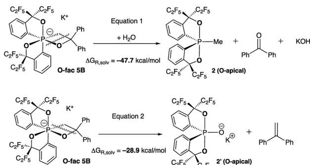
Scheme 5 Calculated fragmentation pathways of O-mer 5B in the presence and absence of water at the (SMD:thf)ω-B97XD/def2-tzvp//ω-B97XD/def2-svp level. 49
