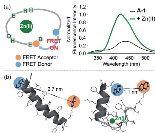
Fig. 2 FRET response of A-1 to Zn(II) and proposed structures of metal-free and Zn(II)-bound A-1. (a) Change in fluorescence upon incubation of A-1 (black) with Zn(II) (green). Conditions: [A-1] = 0.5 \mu M; [ZnCl 2 ] = 100 \mu M; \lambda_{\text{ex}} = 280 nm. (b) Proposed structures of metal-free A-1 (left) and Zn(II)-bound A-1 (right). The structures were generated by modifications of the previously reported structures of metal-free A \beta (PDB: 1AMC) 27 and Zn(II)-bound A \beta (PDB:1ZE9). 28 The approximate distances between the FRET donor and acceptor were indicated with dashed lines.
