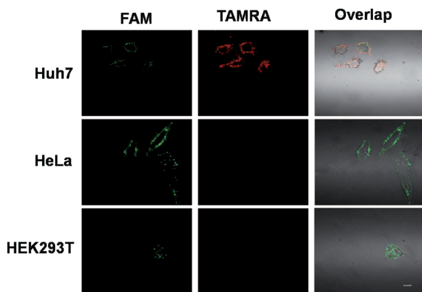
Fig. 4 The fluorescence images of the cascaded logic DNA circuits with three cell lines: Huh 7, HeLa and HEK 293 T. The imaging was performed with a 60× oil immersion objective. Green field = FAM fluorescence and red field = TAMRA fluorescence. The scale bar is 10 μm.
