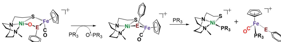
Fig. 7 Reaction of complex 2+\text{O} ( \text{E} = \text{Se} ) or 1+\text{O} ( \text{E} = \text{S} ) with O-abstrating agents, \text{PR}_3 ( \text{R} = \text{Me} or o -tolyl).
