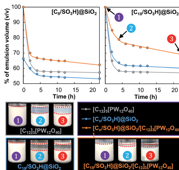
Fig. 5 Evolution of the emulsion volume fraction (S.D. = 2%) as a function of the storage time at 60 °C for the water/toluene emulsions (1/1 v/v) stabilized by [C_n/SO_3H]@SiO_2 and [C_{12}]_3[PW_{12}O_{40}] NPs or a mixture of both NPs (3.6 wt%, \phi = 0.5 , 11 500 rpm). The insets show the W/O emulsions stabilized by [C_{18}/SO_3H]@SiO_2 and/or [C_{12}]_3[PW_{12}O_{40}] NPs.
