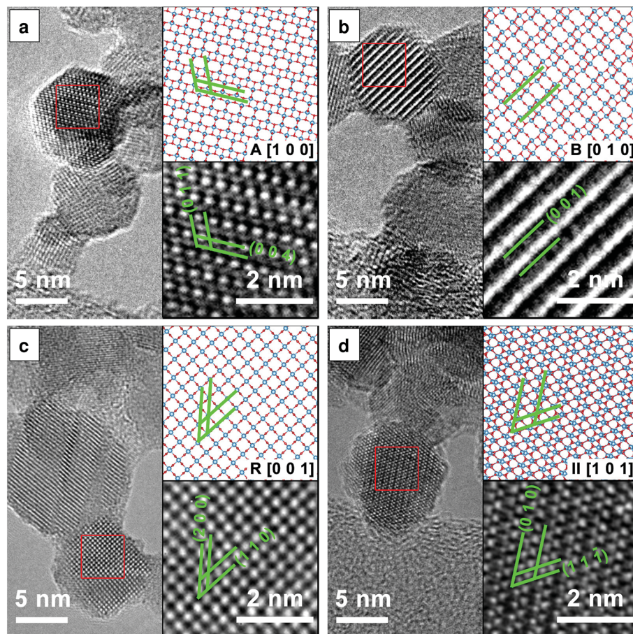
Fig. 3 HRTEM images of the four \text{TiO}_2 polymorphs identified at different flame equivalence ratios \phi : (a) anatase, \phi = 0.50 , (b) \text{TiO}_2 -B, \phi = 0.50 , (c) rutile, \phi = 1.00 , (d) \text{TiO}_2 -II, \phi = 1.67 . The bottom inset is an enlarged view of the area in the red square. The top inset is a ball-and-stick representation of the particular polymorph with the same orientation as in the HRTEM image (Ti: blue, O: red). The relevant crystal planes are annotated in green.
