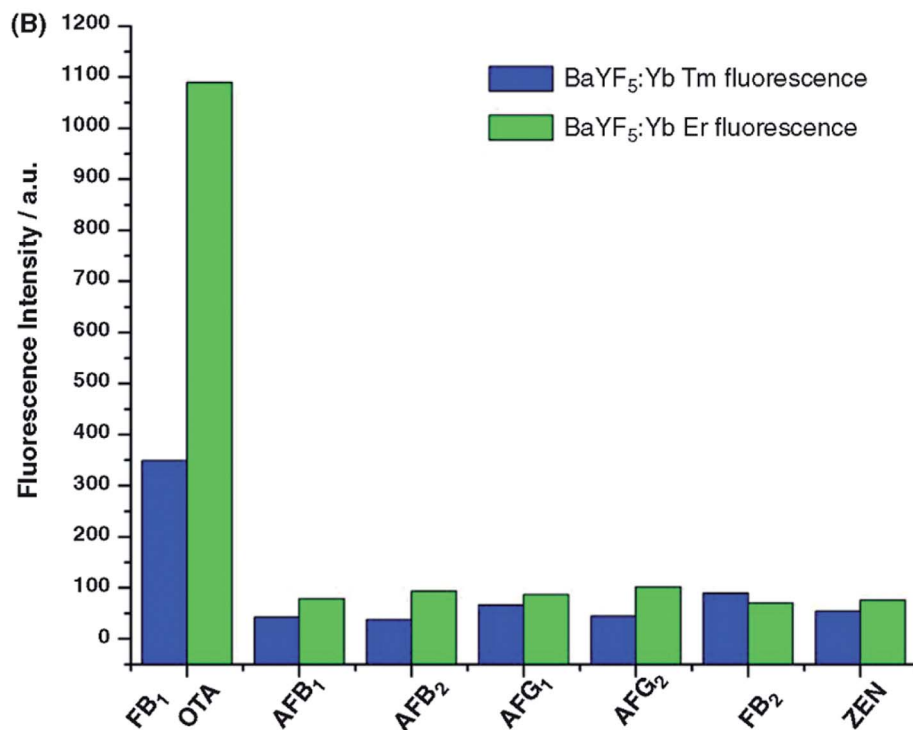
Fig. 35 (A) Schematic representation of the immobilization of ochratoxin A (OTA) aptamers and fumonisins B1 (FB1) aptamers and their multiplex upconversion FRET between aptamer-UCNPs and GO for detecting OTA and FB1. (B) Fluorescence signal change for different mycotoxins at a concentration of 10 ng mL -1 . FB1 and OTA show a significant increase in fluorescence intensity compared with other mycotoxin homologs, including AFB1, AFB2, AFG1, AFG2, fumonisins B2 (FB2) and zearalenone (ZEN), which are commonly found in foods. [Reprinted with permission from ref. 682, S. Wu, N. Duan, X. Ma, Y. Xia, H. Wang, Z. Wang and Q. Zhang, Multiplexed Fluorescence Resonance Energy Transfer Aptasensor Based on Upconversion Nanoparticles and Graphene Oxide for the Simultaneous Determination of Mycotoxins, Anal. Chem. , 2012, 84 , 6263–6270. Copyright© American Chemical Society.]
