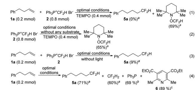
Scheme 3 Mechanistic investigations. a The yields were determined by 19 F NMR spectroscopy based on 1a (0.2 mmol); b isolated yield based on [\text{Ph}_3\text{P}^+\text{CF}_2\text{H}]\text{Br}^- ; c isolated yield based on the Hantzsch ester.
