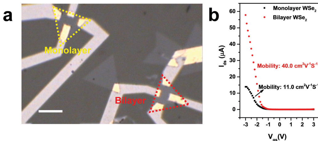
Fig. 4 (a) Optical image of monolayer/bilayer WSe 2 crystals for the device fabrication. Scale bar: 15 \mu\text{m} ; (b) I_{\text{ds}} as a function of V_{\text{gs}} for monolayer/bilayer WSe 2 crystals device. V_{\text{d}} = 0.5 \text{ V} , C_{\text{g}} = 5.0 \text{ } \mu\text{F cm}^{-2} . The mobility of monolayer and bilayer crystals were measured to be 11.0 and 40.0 \text{cm}^2 \text{ V}^{-1} \text{ s}^{-1} , respectively.
