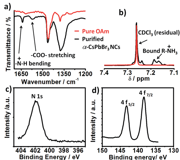
Fig. 2 (a) FTIR spectra of the purified CsPbBr 3 NCs (black) compared to pure oleyl amine (red). (b) ^1\text{H} NMR of purified \alpha -CsPbBr 3 NCs in CDCl 3 (black) compared to pure oleyl amine (red). (c) XPS N 1s and (d) Pb 4f core level XPS spectra of CsPbBr 3 NCs.
